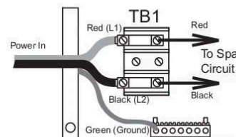
Figure 9 3-Wire, 240 VAC Connection (Hard-wired connections only)
